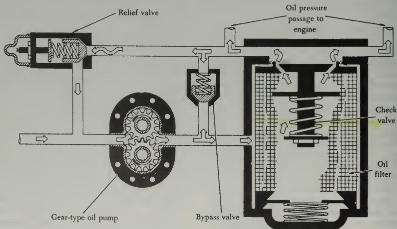
FIGURE 6-4. Engine oil pump and associated units.
